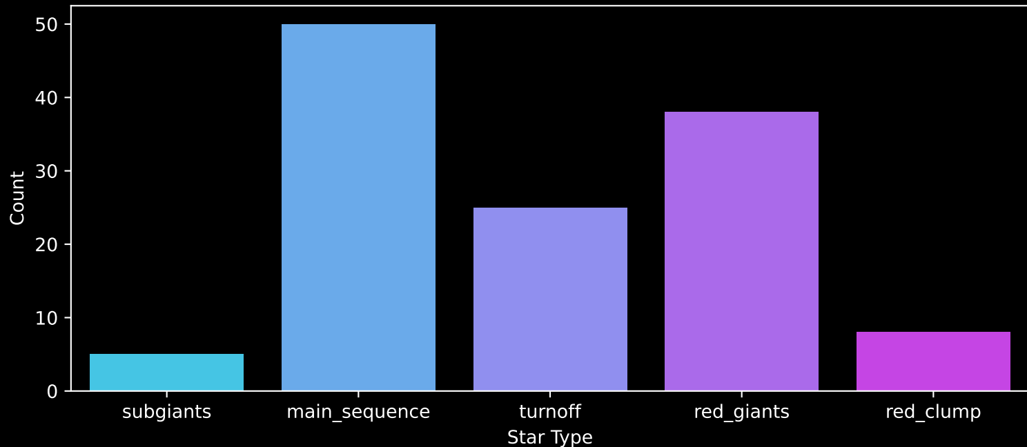
APOGEE DR17 Field: [278-37-O_TESS] Count plot of Star Type
