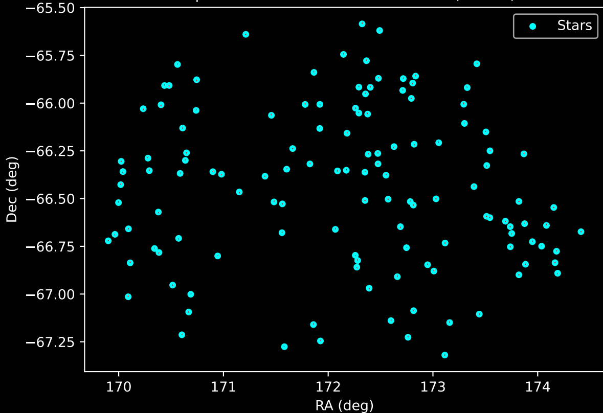
APOGEE DR17 Field: [278-37-O_TESS] Proper Motion Vectors for Gaia Star Field (n= 126)
