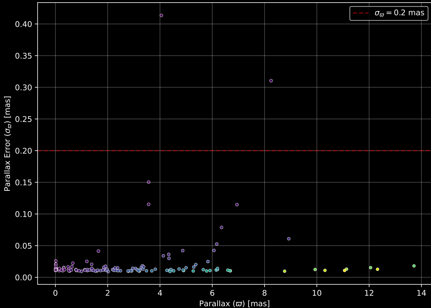
APOGEE DR17 Field: [278-37-O_TESS] Parallax Quality (n= 126)
