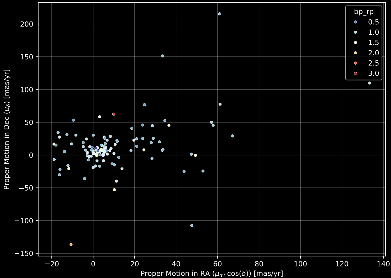
APOGEE DR17 Field: [278-37-O_TESS] Proper Motion Diagram (n= 126)
