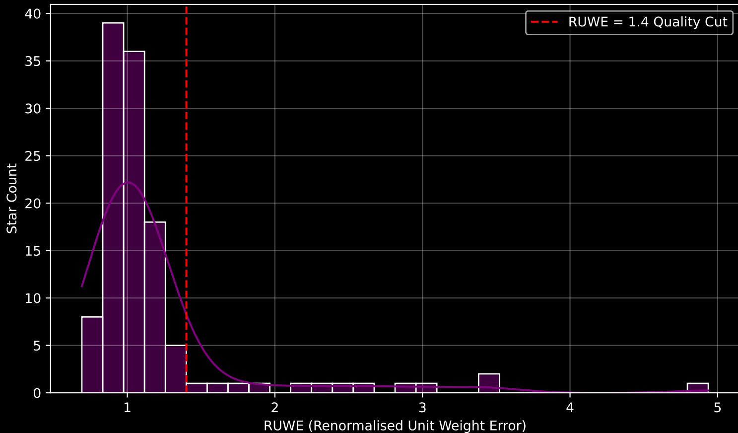
GAPOGEE DR17 Field [278-37-O_TESS] RUWE Distribution (n= 119)
