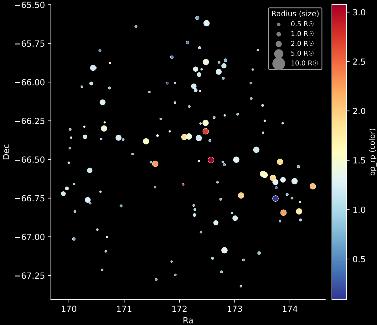
APOGEE DR17 Field: [278-37-O_TESS] Stars: 126
