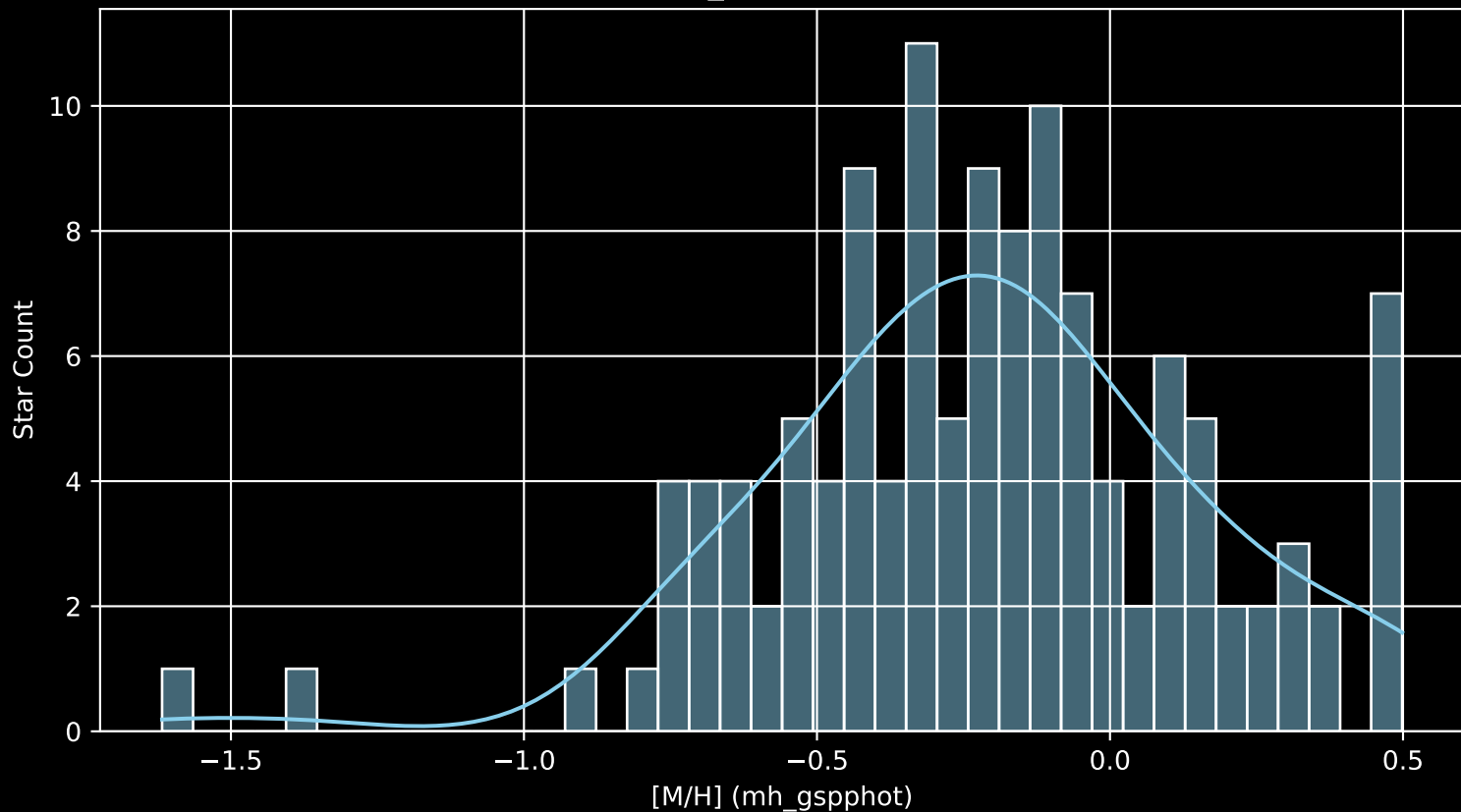
APOGEE DR17 Field: [278-37-O_TESS [M/H] (mh_gspphot) (n= 123)
